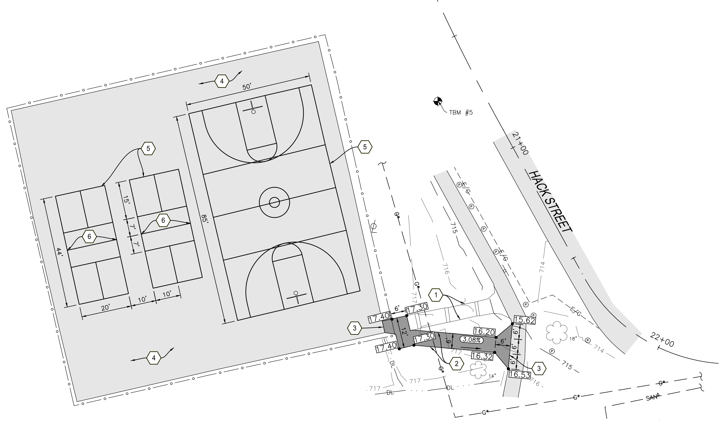
PROJECT 3: COURT SIDEWALK PROJECT 4: BASKETBALL & PICKLEBALL COURTS SCALE: 1" = 20'
